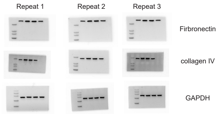
Supplementary Figure 2. The original western blots of Figs. 2, 4, and 5–7. LIN28B , lin28 homolog B; GAPDH , glyceraldehyde-3-phosphate dehydrogenase.
